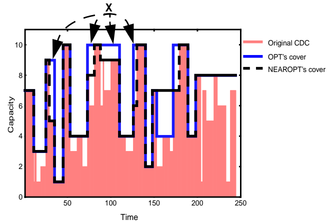
Figure 6: Covers computed by OPT and NEAROPT.
