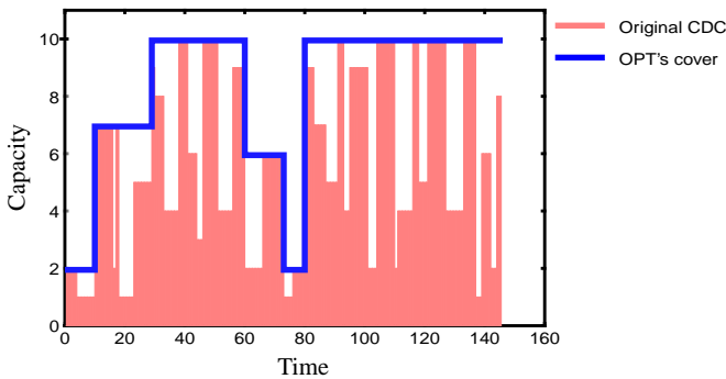
Figure 4: Cost-minimal cover computed by OPT.
