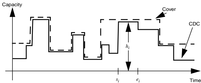
Figure 2: Example CDC with a cover.
